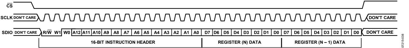
Figure 63. Serial Control Port Write—MSB First, 16-Bit Instruction, Two Bytes of Data
